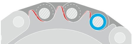
Additional wear on sprockets
