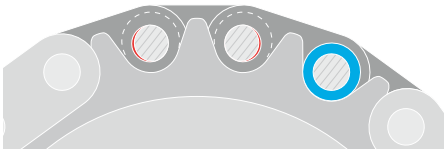
Timing chains can lengthen as a result of wear on the pins and inside the ferrules.
