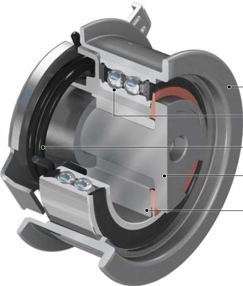
Semi-automatic tensioning pulley with double eccentric
